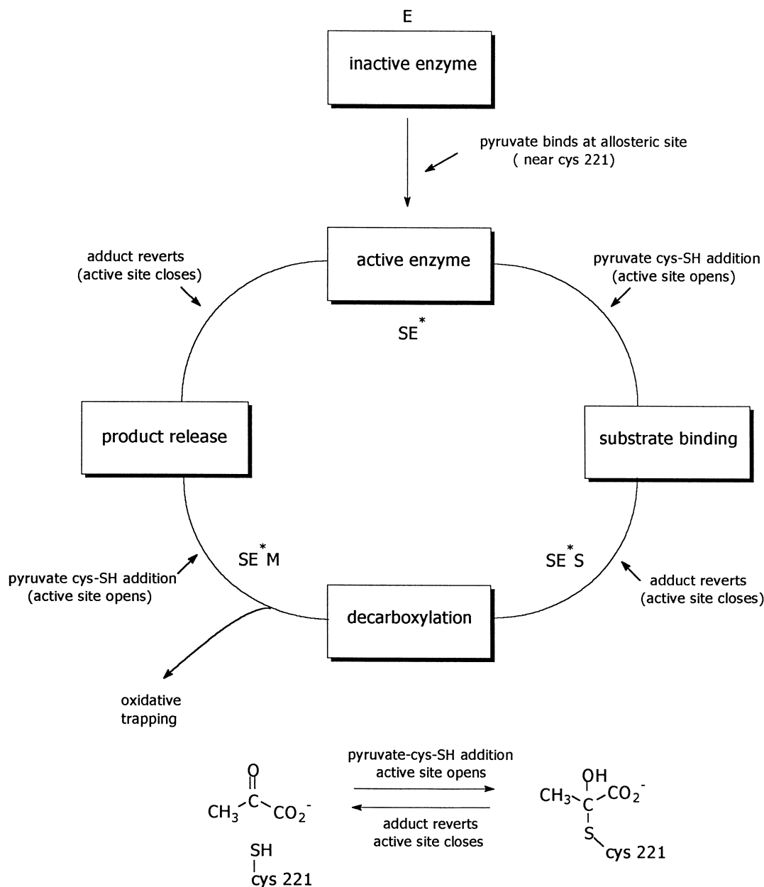
Figure 2. The active-site access model for the hysteretic, allosteric regulation of SCPDC. The slow, hysteretic activation is assumed to involve placement of the 'regulatory pyruvate' at the allosteric site of the free enzyme E, in which active-site access is denied. Binding at the allosteric site is indicated by writing S to the left of E, and completion of the slow activation process by the asterisk in SE*. During the catalytic cycle, addition of the sulfhydryl group of Cys-221 to the keto group of the regulator opens the active site and elimination recloses it. The substrate enters the active site of SE* during an open period to produce SE*S. The active site is presumed closed during decarboxylation, which yields SE*M. Protonation and elimination then gives the product complex and product departs during an open period.
