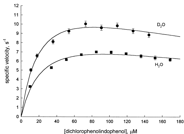
Figure 4. Specific velocity of the oxidative diversion reactions versus oxidant concentration at a saturating concentration of pyruvate. Filled circles refer to reaction in deuterium oxide, filled squares to reaction in protium oxide. The solid lines are plots of eq (1) with the parameters shown in Table 1.
