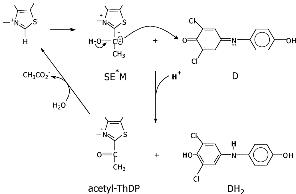
Figure 3. The concept of paracatalytic oxidative diversion during SCPDC action. 19 The oxidant dichlorophenolindophenol ( D ) traps the product of decarboxylation, the 'second carbanion' SE*M. Oxidation leads to acetyl-ThDP which then hydrolyzes to release acetate and complete the catalytic cycle.
