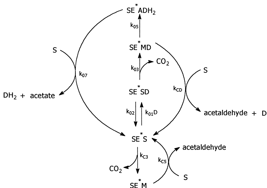
Figure 5. Kinetic model for the oxidative-diversion reaction under conditions of saturating pyruvate. Subscripts c refer to the normal catalytic cycle, and subscripts o to the oxidative diversion. Note that rate constants are in some cases aggregate rate constants for several serial events. The normal catalytic cycle connecting SE^*S and SE^*M is shown at the bottom (free or unactivated enzyme are not present because of the saturating concentration of S ). The oxidative-diversion branch extends upward from SE^*S , beginning with entry of D into the active site and continuing with decarboxylation in the presence of D to generate SE^*MD . The mechanism again branches, with protonation of the 'second carbanion' and elimination yielding acetaldehyde while oxidative diversion competitively generates a complex SE^*ADH_2 . This complex contains in the active site DH_2 and acetyl-ThDP; the latter hydrolyzes and acetate and DH_2 are released.
