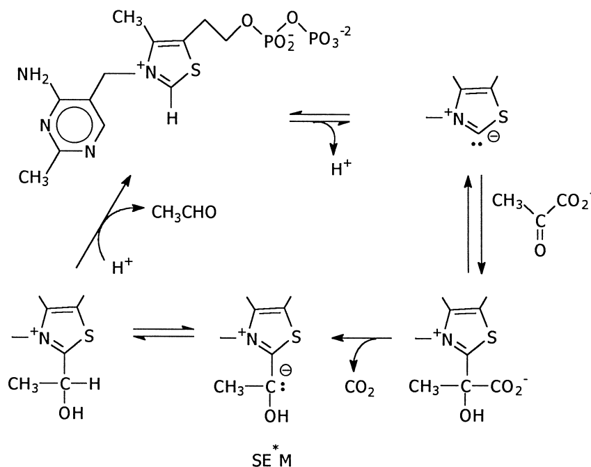
Figure 1. The normal catalytic cycle for SCPDC. Note the structure of thiamin diphosphate (ThDP) with a diphosphate arm and a pyrimidine arm. Ionization of the acidic C2–H bond leads to the ‘first carbanion’. Addition of this species to the substrate pyruvate produces decarboxylation and formation of the ‘second carbanion’. Protonation of the latter and elimination to form acetaldehyde completes the catalytic cycle. The ‘second carbanion’ is denoted SE*M in the system 20 used herein for mechanistic descriptions (see Figs 2 and 5).
